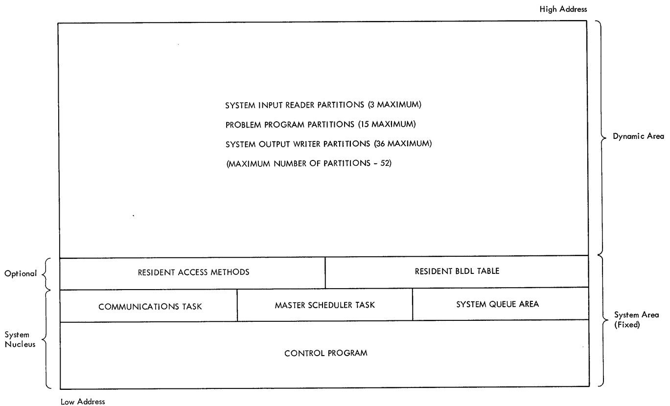
Figure 1. Main Storage Organization
