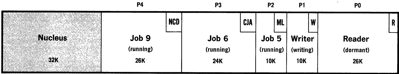
Figure 10. Contents of Main Storage With All Partitions Active
