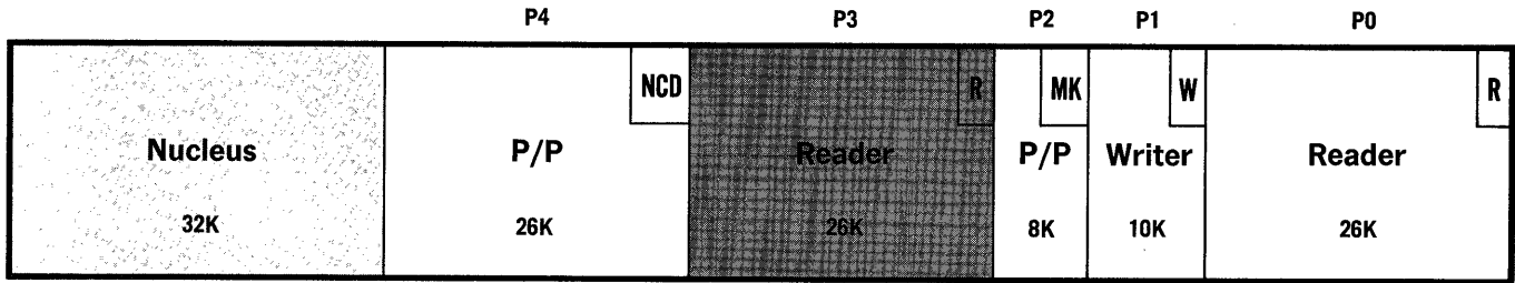
Figure 16. Partition Recovery With Identity Change
