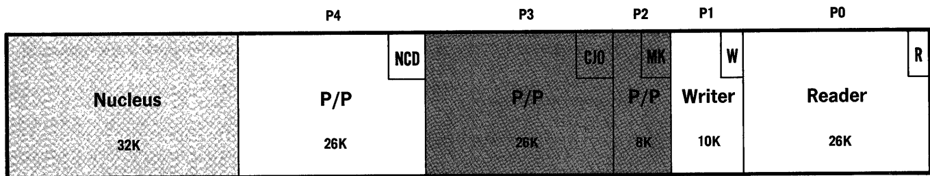
Figure 15. Partition Configuration After Recovery
