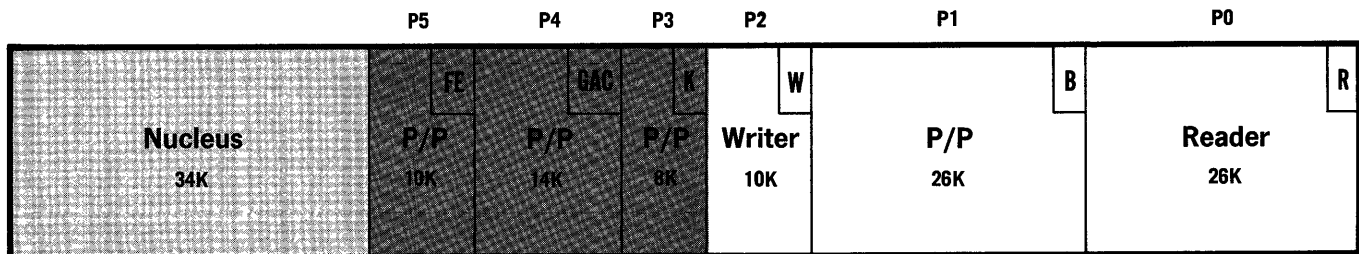
Figure 21. Sample 128K Small Partition Configuration
