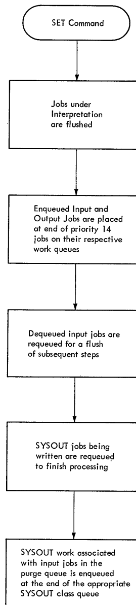
Figure 20. Restarting the System
