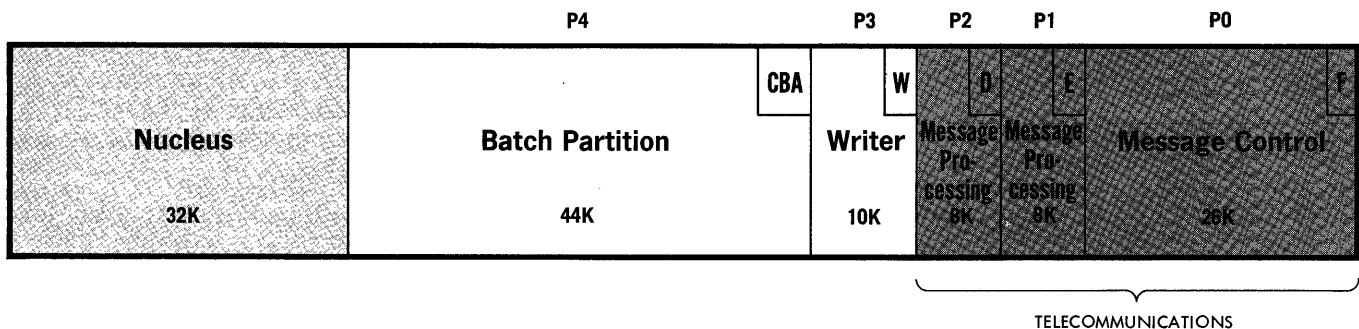
Figure 22. Sample 128K Telecommunications-Oriented Configuration
