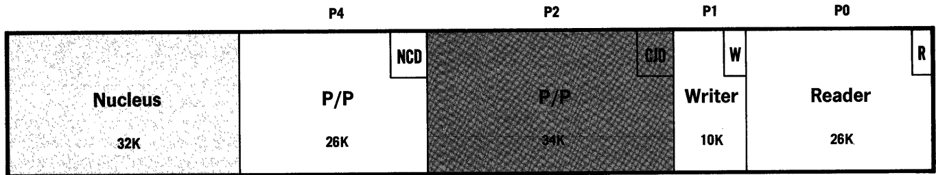
Figure 14. Partition Identification After Combination
