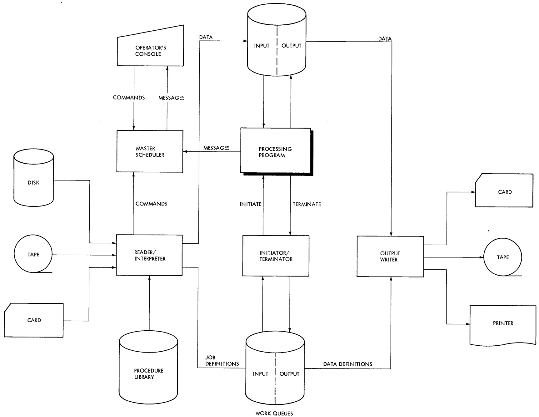
Figure 19. The MFT II System
