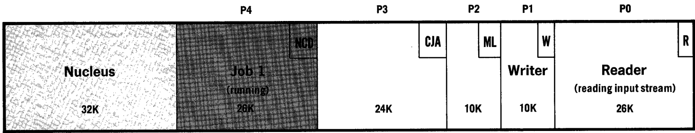
Figure 8. Contents of Main Storage After First Job Has Been Scheduled
