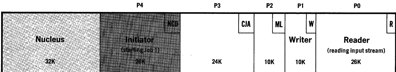
Figure 7. Contents of Main Storage After START Commands
