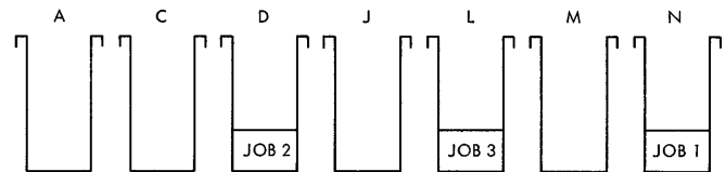
Figure 6. Input Work Queues After First Three Jobs Have Been Entered
