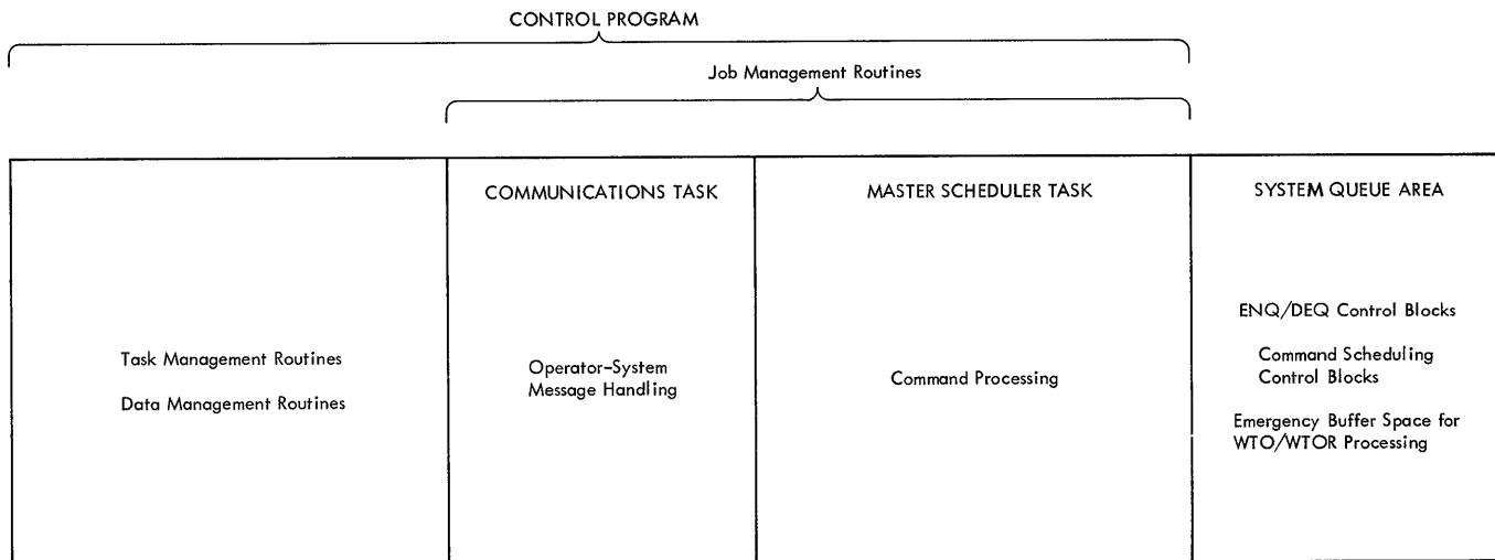
Figure 12. Components of the Nucleus
