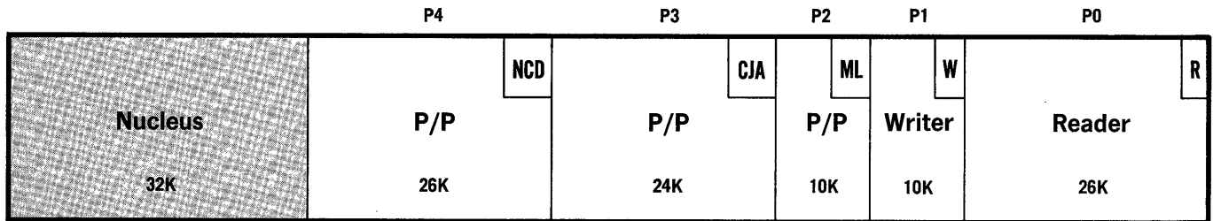
Figure 11. Sample Five-Partition Configuration
