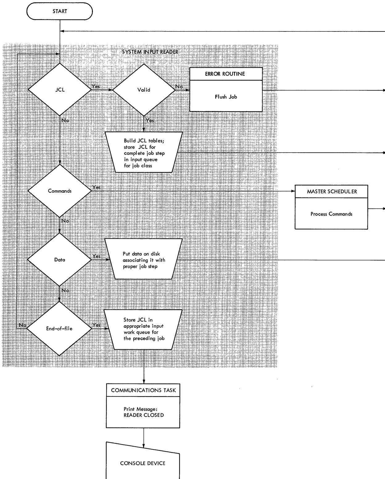
Figure 18. System Input Reader Processing
